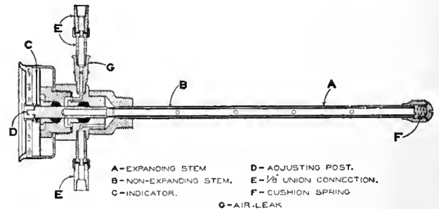
FIG. 3. SECTION SHOWING CONSTRUCTION OF AN INSERTION THERMOSTAT
